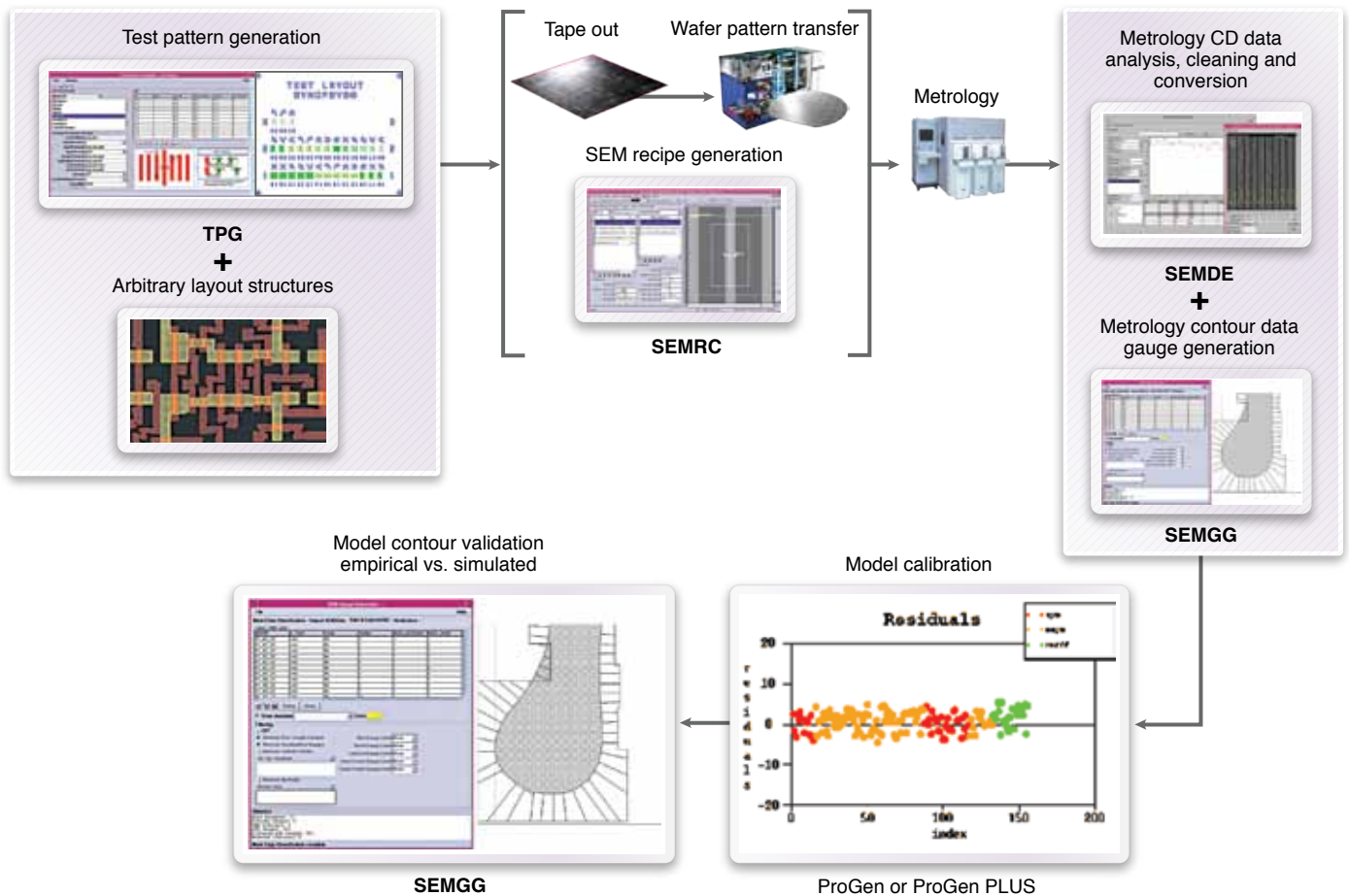
Figure 1: Model generation flow
